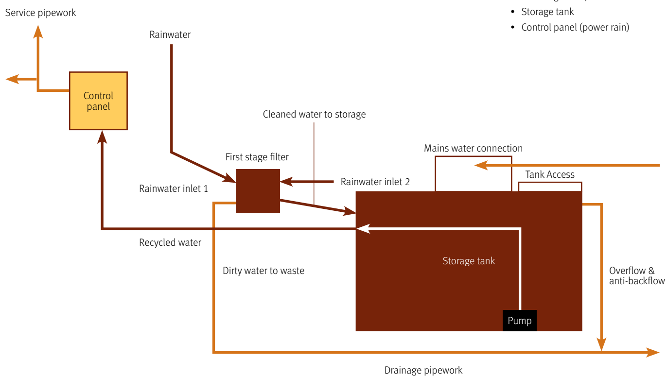
Figure 3 → Principles of a direct system
