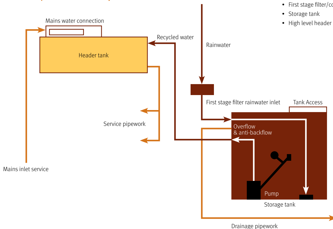
Figure 2 → Principles of an indirect system
